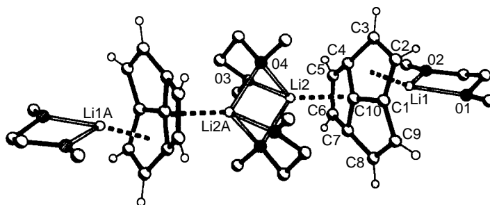
Fig. 8.P17. Crystal structure of \text{Li}_2(\text{DME})_2\text{acepentalenediide} . Reproduced from Angew. Chem. Int. Ed. Engl. , 34 , 1492 (1995), by permission of Wiley-VCH.
