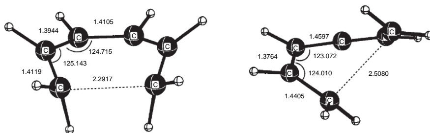
Fig. 10.26. Disrotatory (left) and conrotatory (right) transition structures for 1,3,5-hexatriene electrocyclic cyclization from MP2/CAS/6-311+G( d,p ) calculations. Reproduced from J. Phys. Chem. A , 103 , 2878 (1999), by permission of the American Chemical Society.
