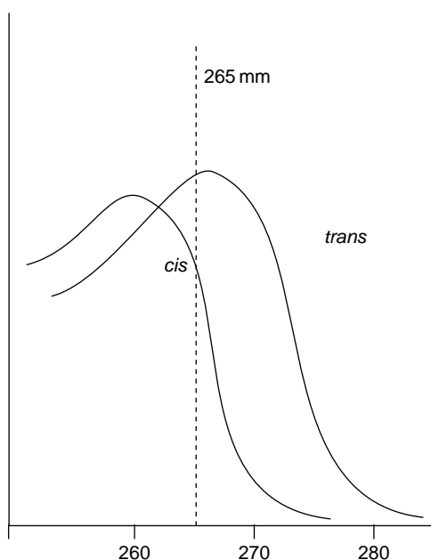
Fig. 12.4. Absorption spectra of a cis-trans isomer pair.
