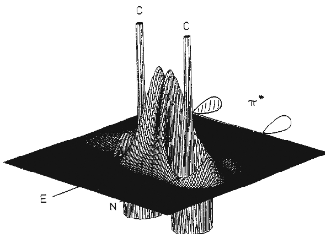
Fig. 1.40. Perspective of Laplacian -\nabla^2\rho_{c,r} of ethene in a plane perpendicular to the molecular plane. From E. Kraka and D. Cremer in The Concept of the Chemical Bond , Z. B. Maksic, ed., Springer-Verlag 1990, p. 533.
