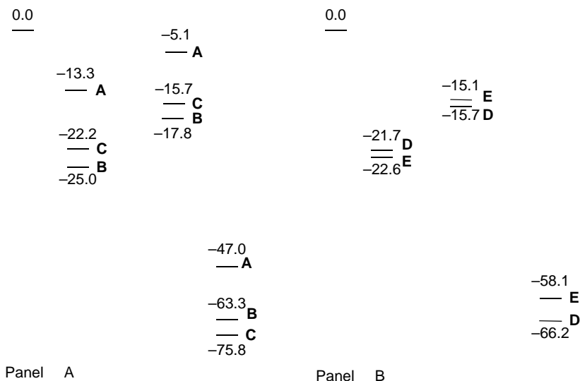
Fig. 7.14. Panel A: Relative \Delta H of reactant complex, transition structure, and products at 0^\circ\text{C} (including ZPE correction) for acetone (A), methoxyacetone (B), and methoxyacetaldehyde (C). Panel B: Relative \Delta H at 0^\circ\text{C} (including ZPE correction) for 3-methoxypropanal (D) and 4-methoxy-2-butanone (E). Data from J. Am. Chem. Soc. , 117 , 5055 (1995).
