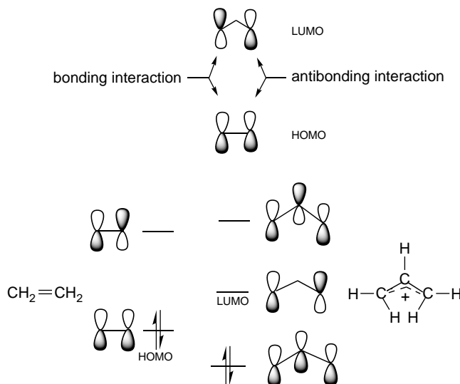
Fig. 1.22. MOs for ethene and allyl cation.
