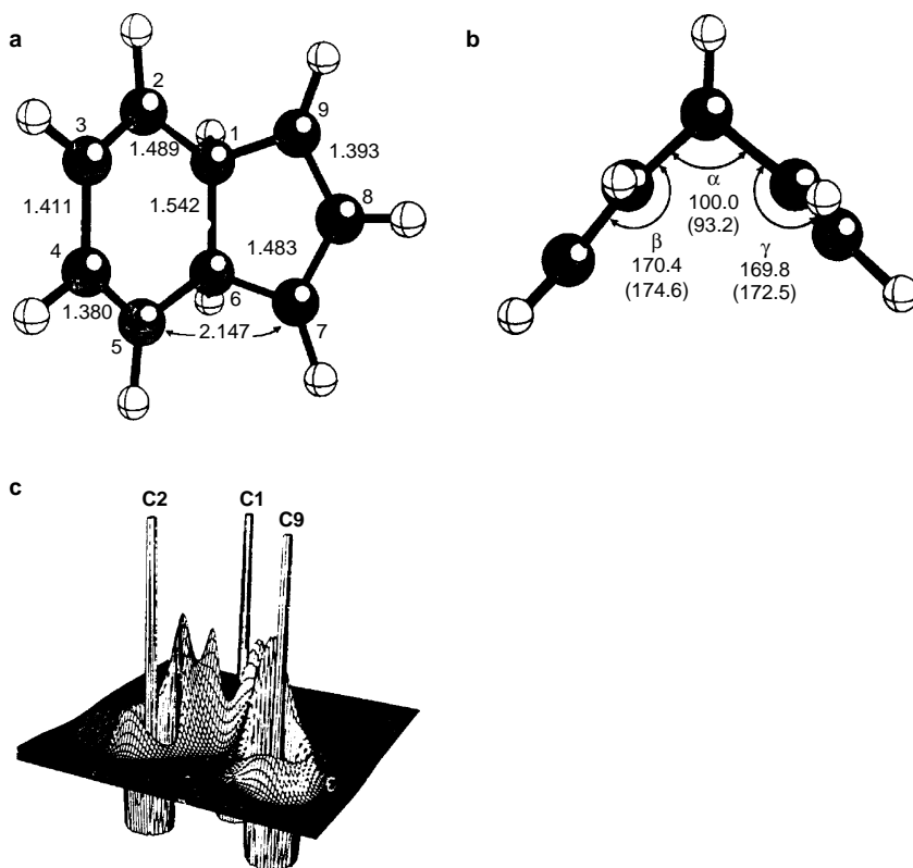
Fig. 8.P14. (a) Bond lengths and (b) inter-ring angles for minimum-energy cation; (c) -\nabla^2\rho(\mathbf{r}) in the \text{C}(1)\text{--}\text{C}(2)\text{--}\text{C}(9) plane. Reproduced by permission of the American Chemical Society Bond Orders: 1,2: 1.04; 2,3:1.59; 3,4: 1.57; 1,6:0.94; 1,9: 1.04; 8,9:1.56; 2,9:0.34.
