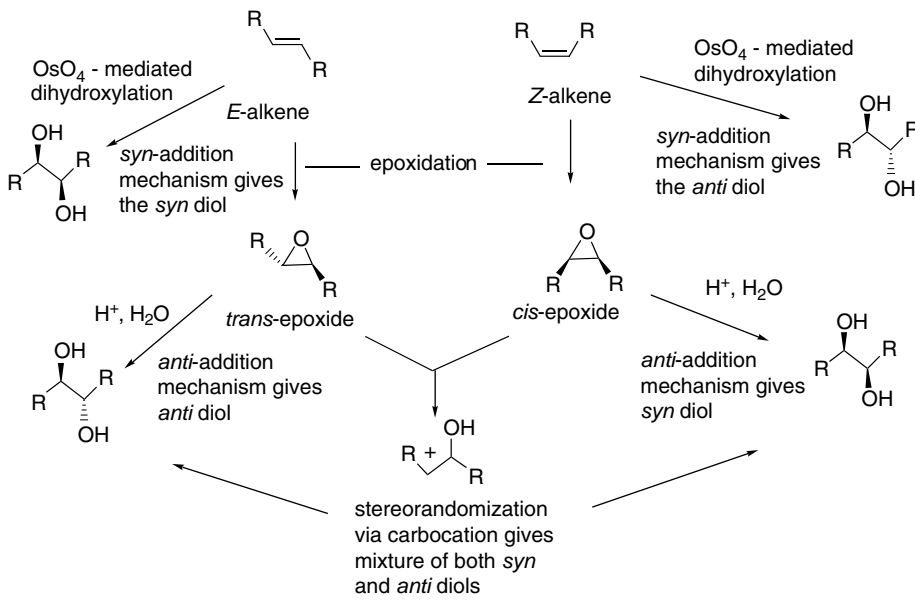
Scheme 2.8. Summary of Stereochemistry of Alkene Dihydroxylation by OsO 4 -Catalysis and Epoxide Ring Opening
