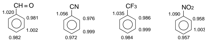
Fig. 9.5. Total \pi -electron density for some substituted benzenes. From HF/STO-3G calculations.
